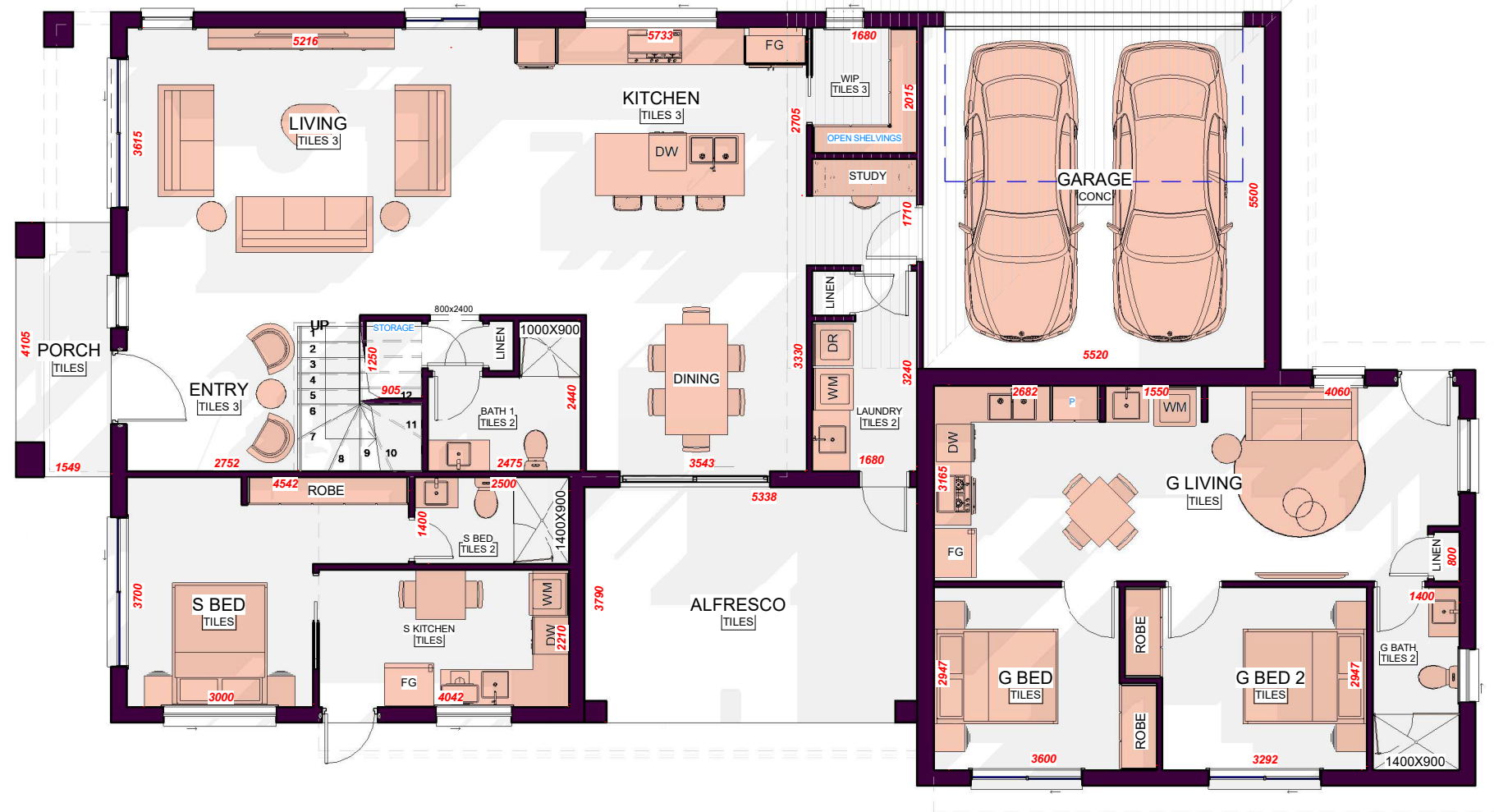
1 .H GROUND FLOOR 1 : 100
