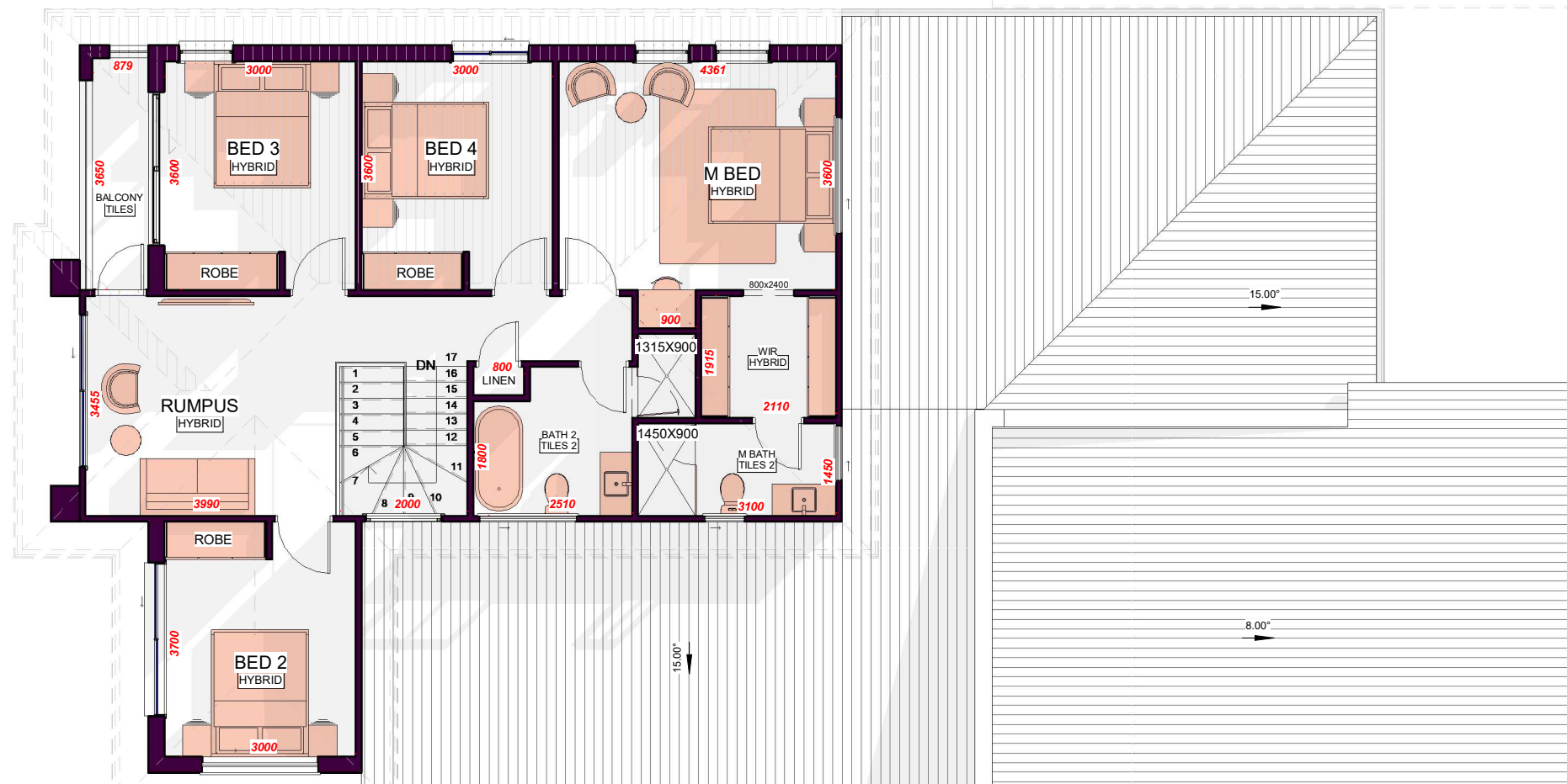
2 .H FIRST FLOOR 1 : 100
